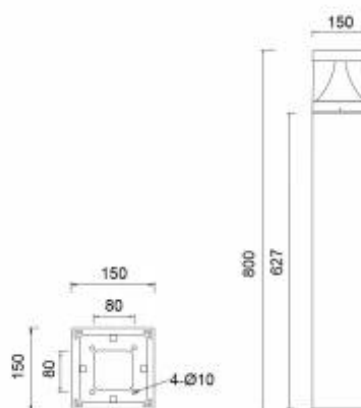
灯具尺寸 Product Dimensions(mm)
