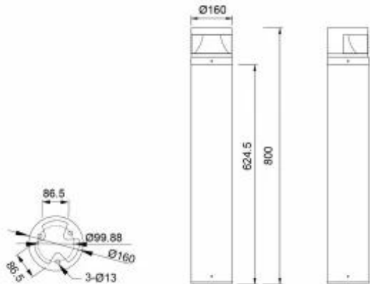
灯具尺寸 Product Dimensions(mm)
