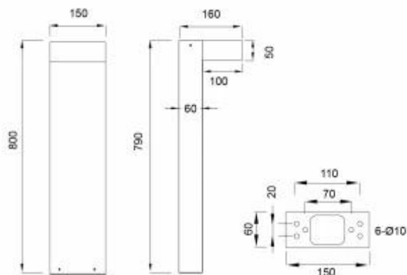
灯具尺寸 Product Dimensions(mm)
