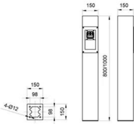
灯具尺寸 Product Dimensions(mm)
