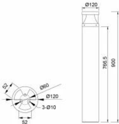
灯具尺寸 Product Dimensions(mm)
