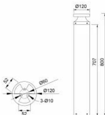
灯具尺寸 Product Dimensions(mm)
