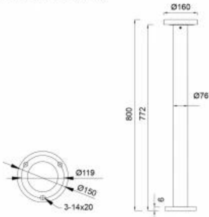
灯具尺寸 Product Dimensions(mm)
