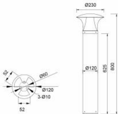
灯具尺寸 Product Dimensions(mm)
