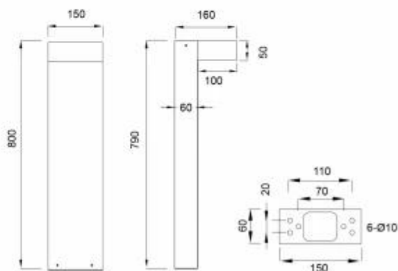
灯具尺寸 Product Dimensions(mm)
