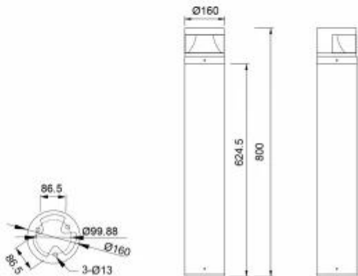
灯具尺寸 Product Dimensions(mm)
