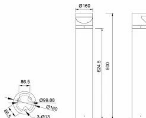
灯具尺寸 Product Dimensions(mm)
