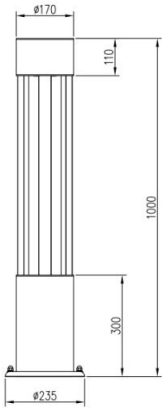
灯具尺寸 Product Dimensions(mm)
