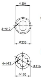
Outer base plate
